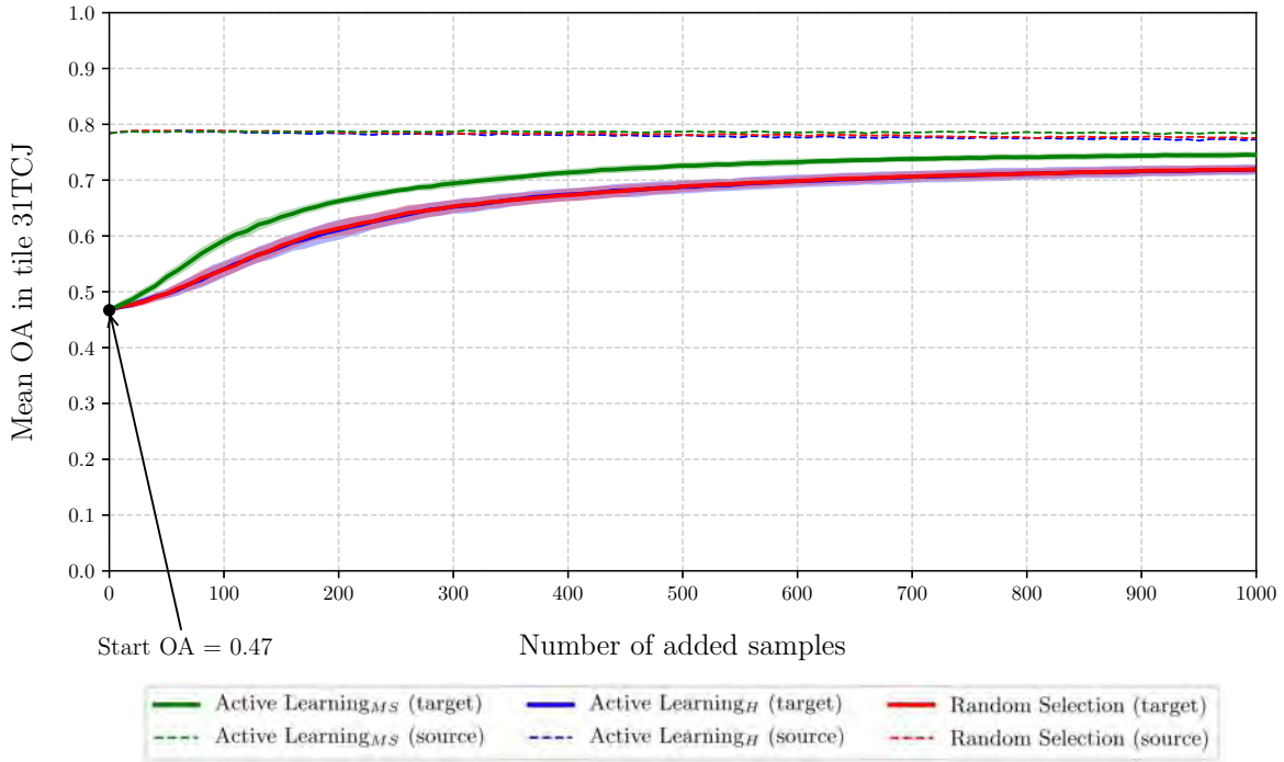
Figure 5.5 – Changes in the average OA scores ( \pm standard deviation) on the south-western target tile (31TCJ) according to the additional number of training samples from the initial model (north-eastern source tile 31UEQ). The average values were based on 30 independent runs for both random sampling (RS in red) and active learning using entropy ( AL_H in blue) or margin sampling ( AL_{MS} in green). Dashed lines show changes in the OA on the north-eastern source tile (31UEQ) with RS (red dashed line), AL_H (blue dashed line) and AL_{MS} (green dashed line).
